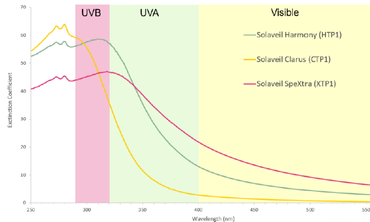
Figure 2 : UV/Visible spectrum for Solaveil Harmony compared to Solaveil Clarus and Solaveil SpeXtra
