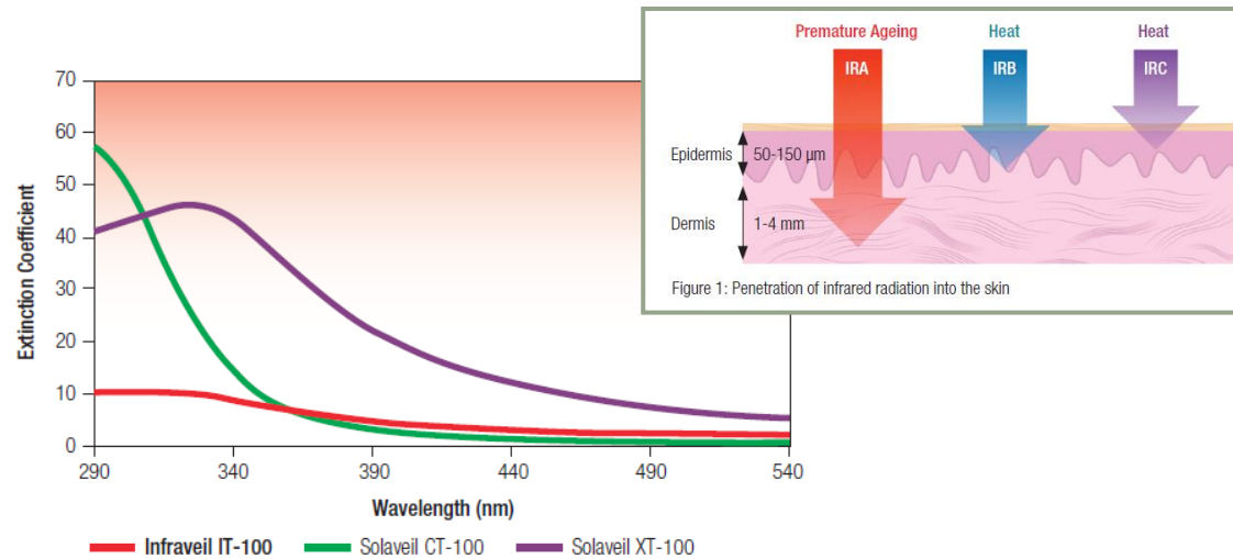
Figure 3: UV/Visible attenuation of Infraveil IT-100 versus Solaveil CT-100 and Solaveil XT-100
