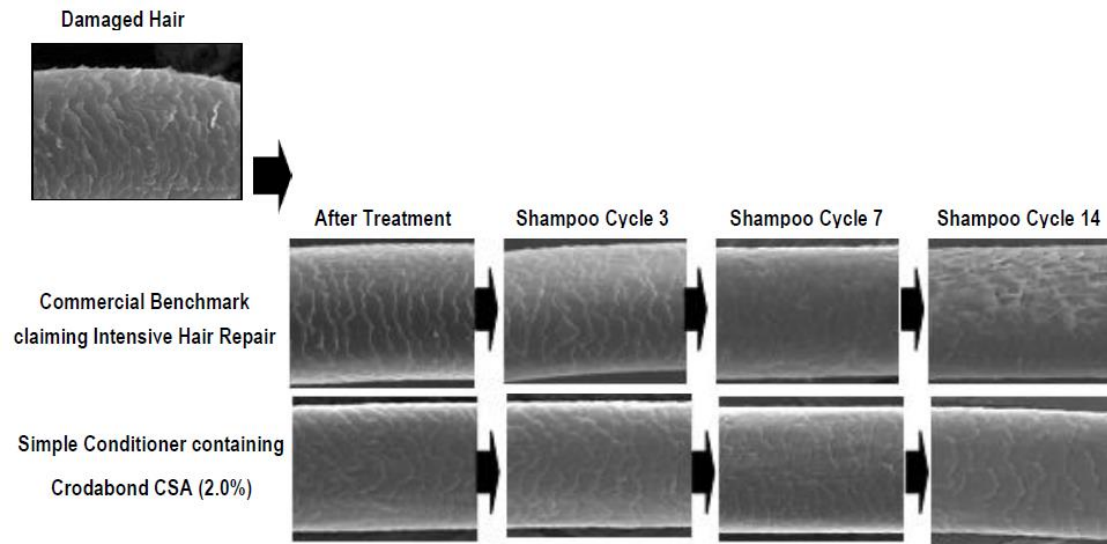
Figure 5: Crodabond CSA can effectively seal down hair cuticles for longer in comparison to a leading commercial conditioner designed for intensive hair repair
